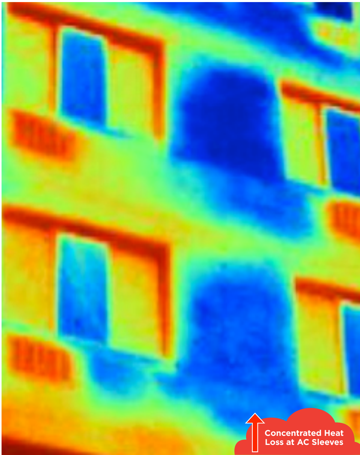
Fig. 1: Infrared image of a building with through-the-wall sleeves (exterior view)
