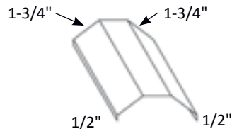
Figure 54.1 #211 Vented Ridge Cap Flashing
