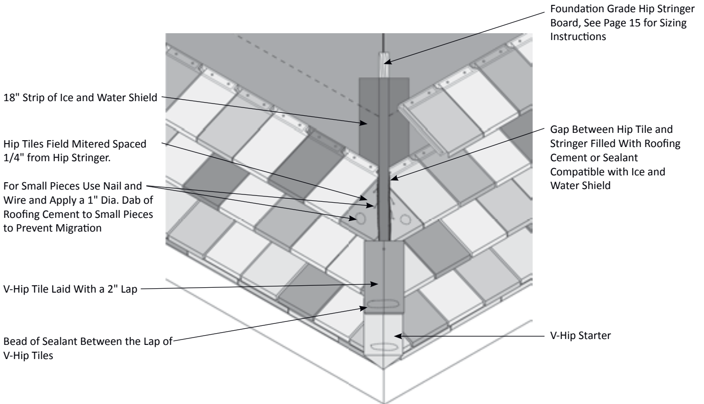
Figure 39.1 V-Hip Detail
