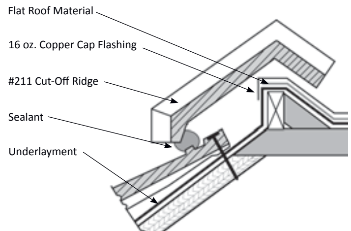
Figure 43.6 Deck Section with #211 Cut-Off Ridge
