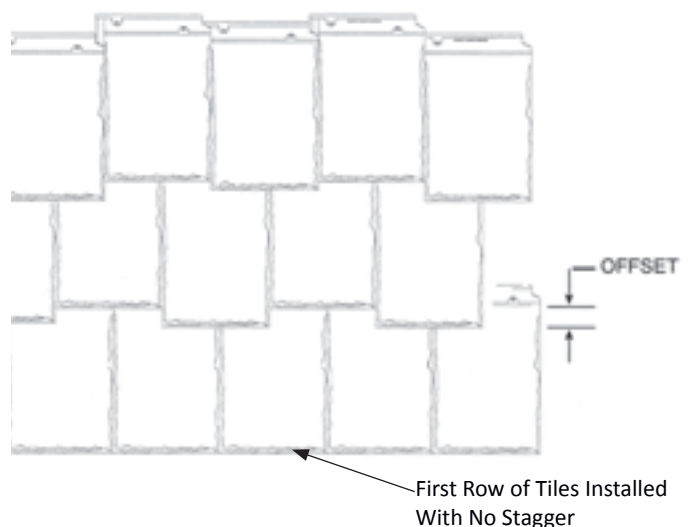
Figure 58.3 Staggered Layout
