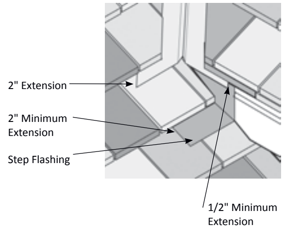
Figure 29.2 Open Valley at Main Roof to Dormer Juncture Close-up
