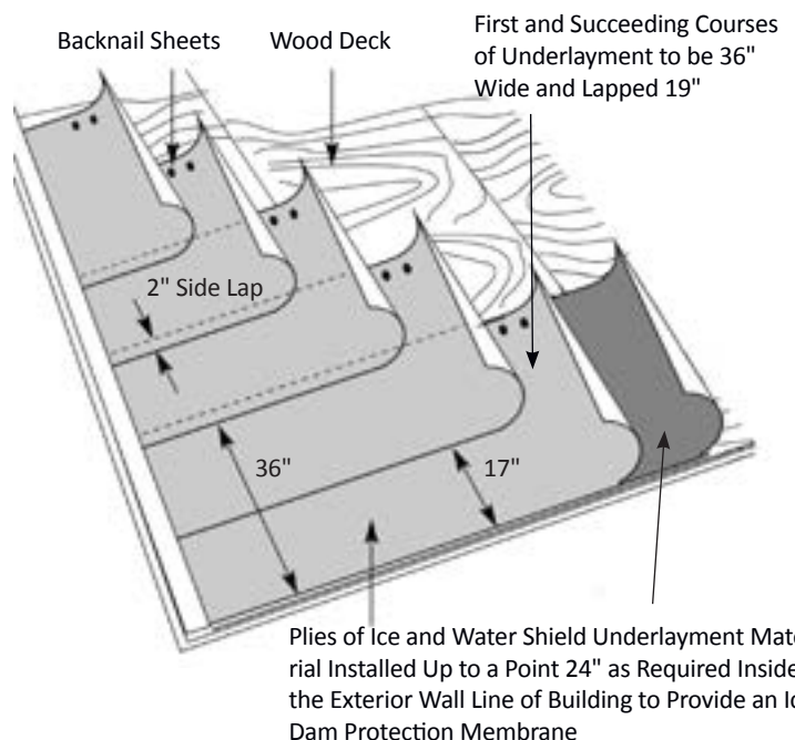
Figure 15.2 Double Sheet Underlayment
