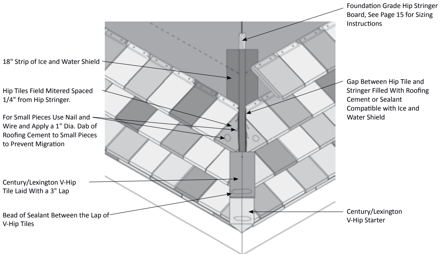
Figure 65.1 V-Hip Detail
