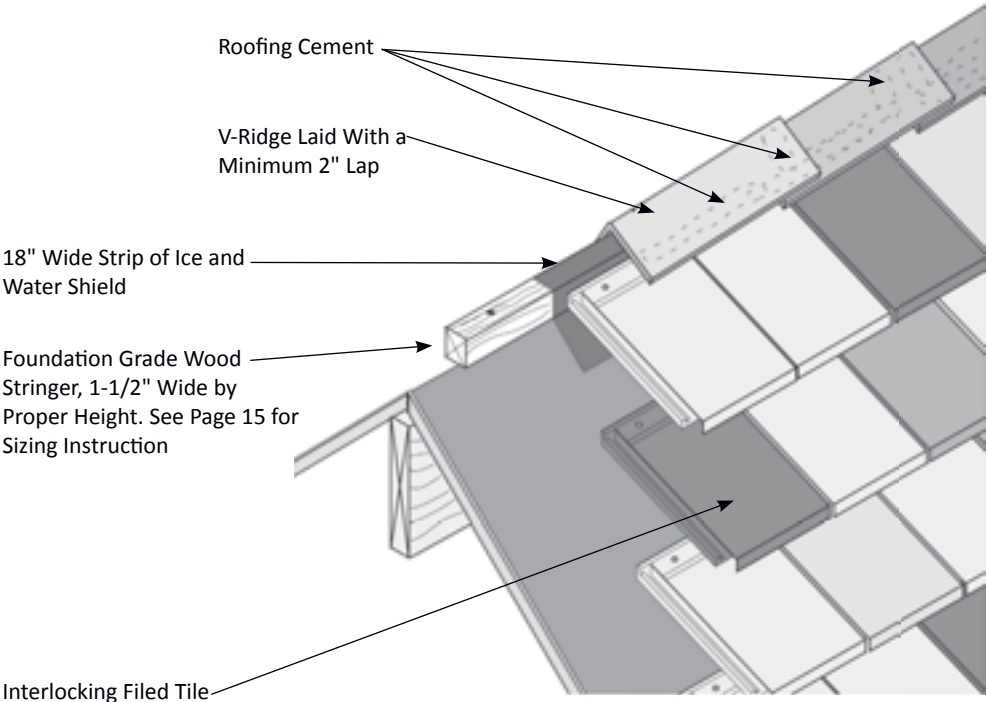
Figure 38.2 V-Ridge Detail
