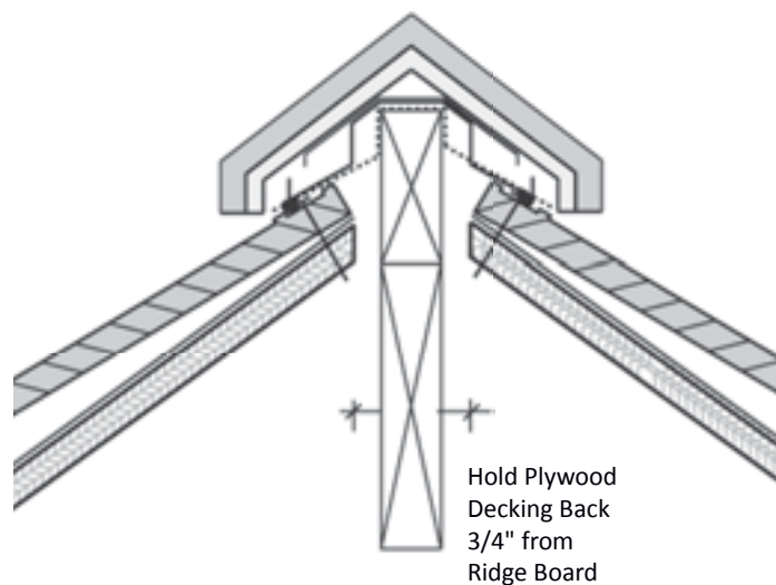
Figure 54.3 #211 Vented Ridge Section
