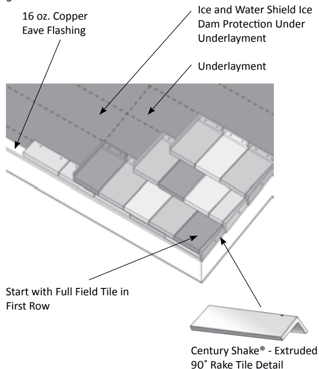
Figure 63.2 Eave Detail
