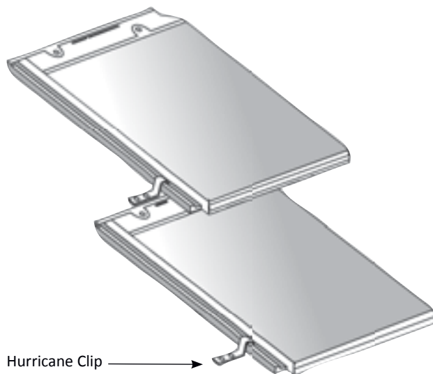
Figure 13.2 Hurricane Clip
