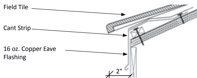
Figure 63.1 Lexington Slate® and Century Shake® Eave Detail with Cant Strip
