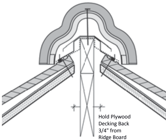
Figure 42.3 #211 Vented Ridge Section
