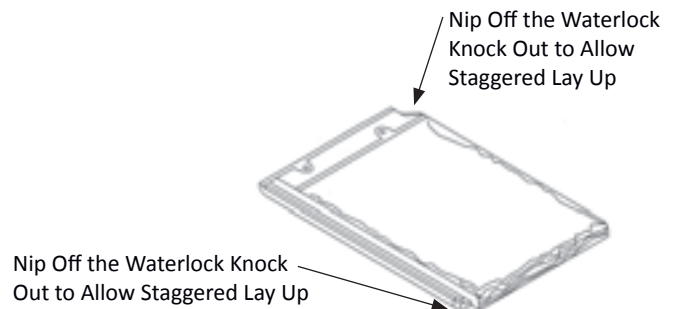
Figure 58.2 Staggered Tile Prep
