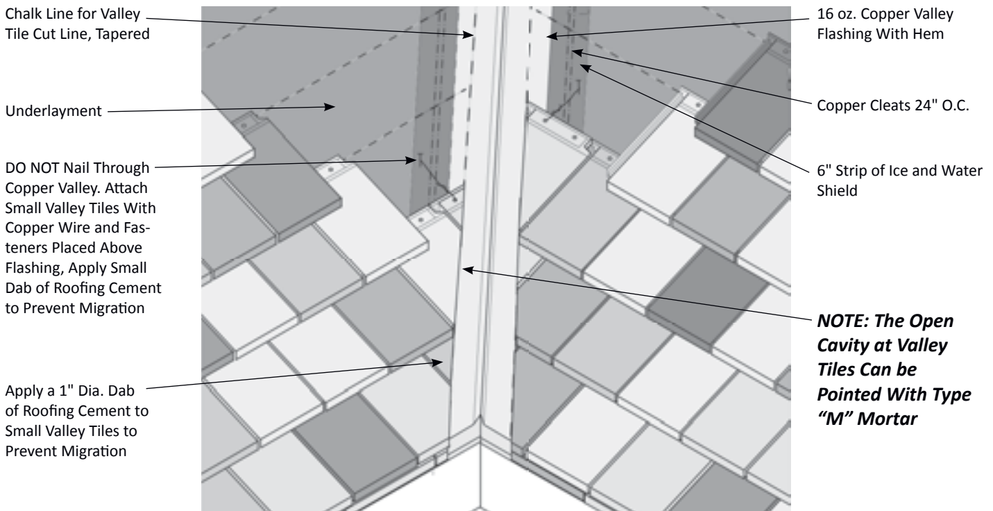
Figure 64.1 Valley Detail
