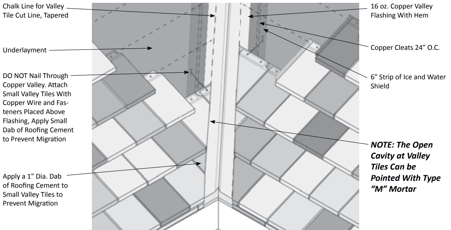
Figure 49.1 Valley Detail
