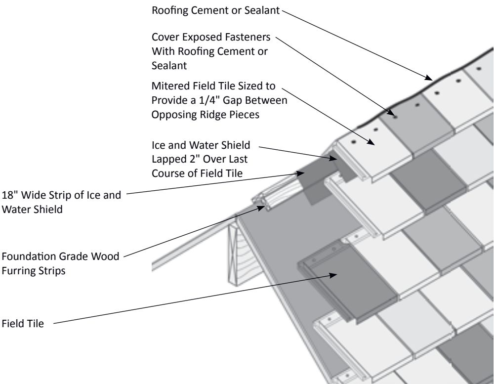
Figure 40.1 Mitered Ridge Detail
