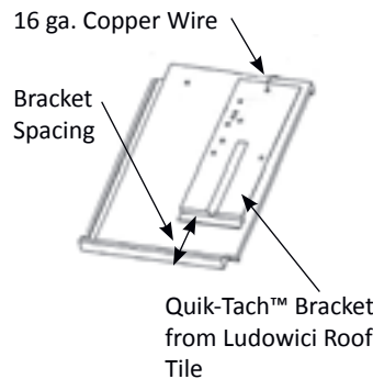
Figure 71.3 Replacement Tile with Quik-Tach™ Bracket
