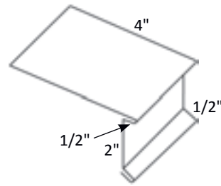
Figure 24.2 Eave Flashing Dimensions
