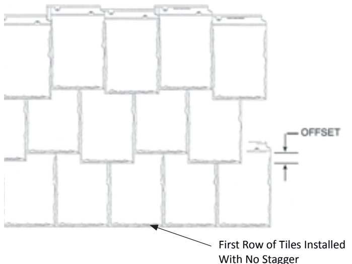
Figure 45.3 Staggered Layout
