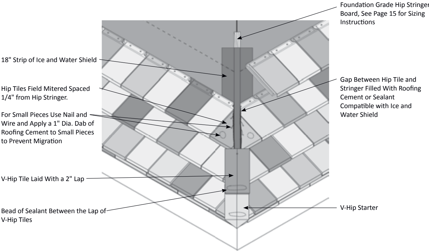
Figure 50.1 V-Hip Detail
