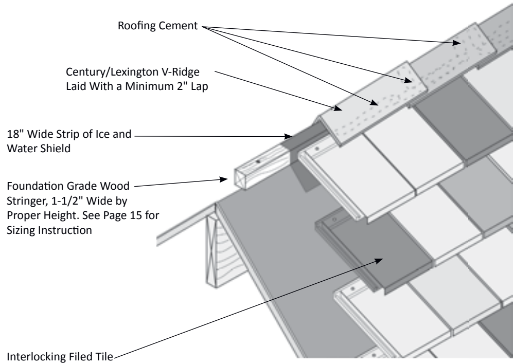
Figure 67.1 V-Ridge Detail
