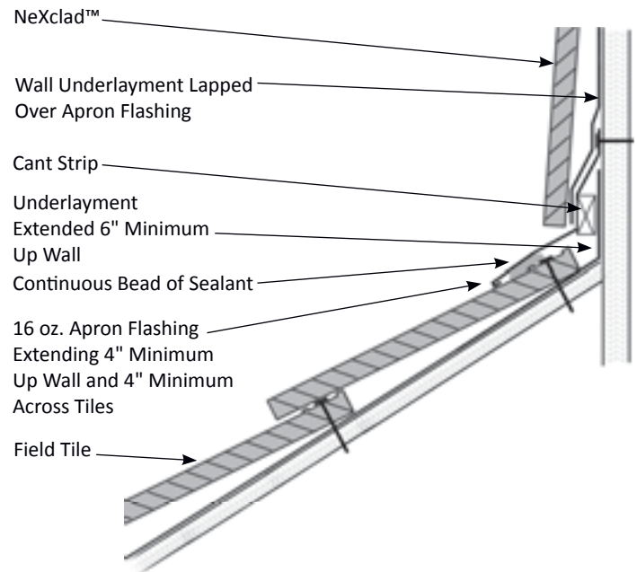
Figure 30.4 Apron Flashing at NeXclad Head Wall
