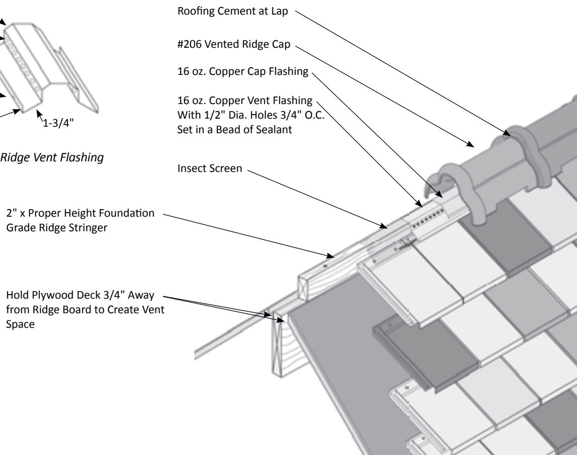
Figure 44.4 #206 Vented Ridge Detail
