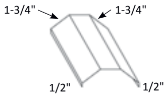
Figure 41.1 #211 Vented Ridge Cap Flashing
