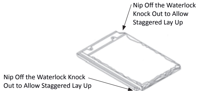
Figure 47.2 Staggered Tile Prep
