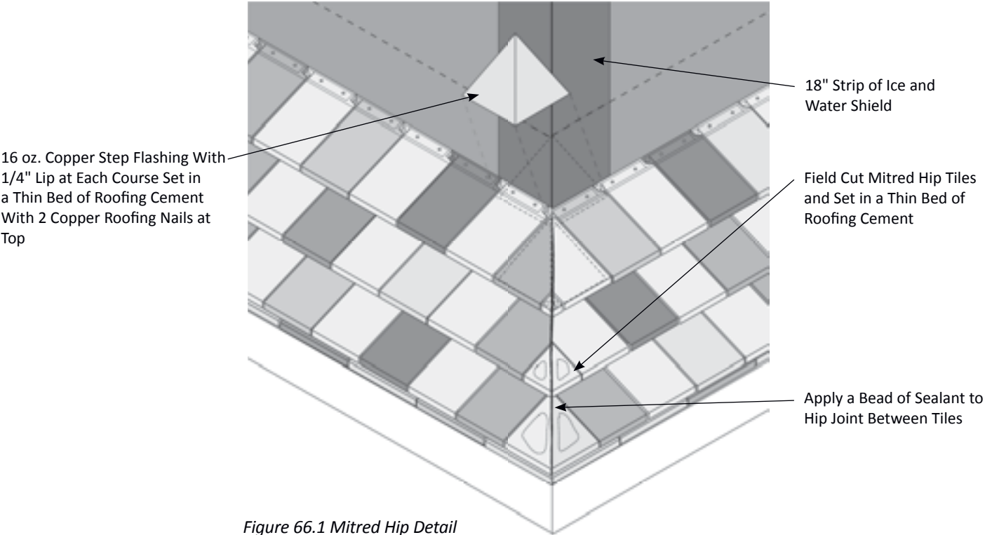
Figure 66.1 Mitered Hip Detail
