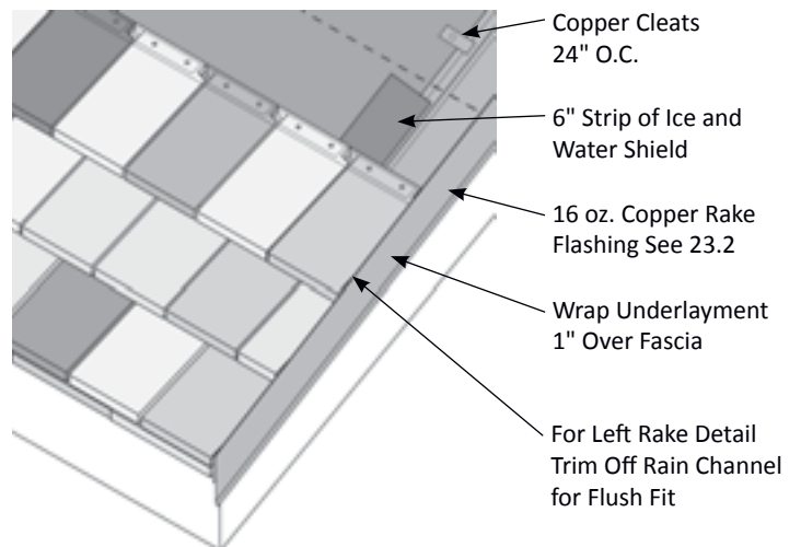
Figure 25.5 Closed Rake Detail
