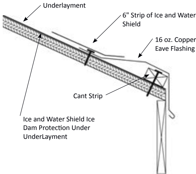
Figure 17.1 Copper Flashing Eave Detail
